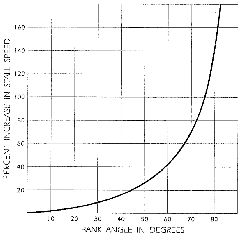
STALL SPEED CHART
