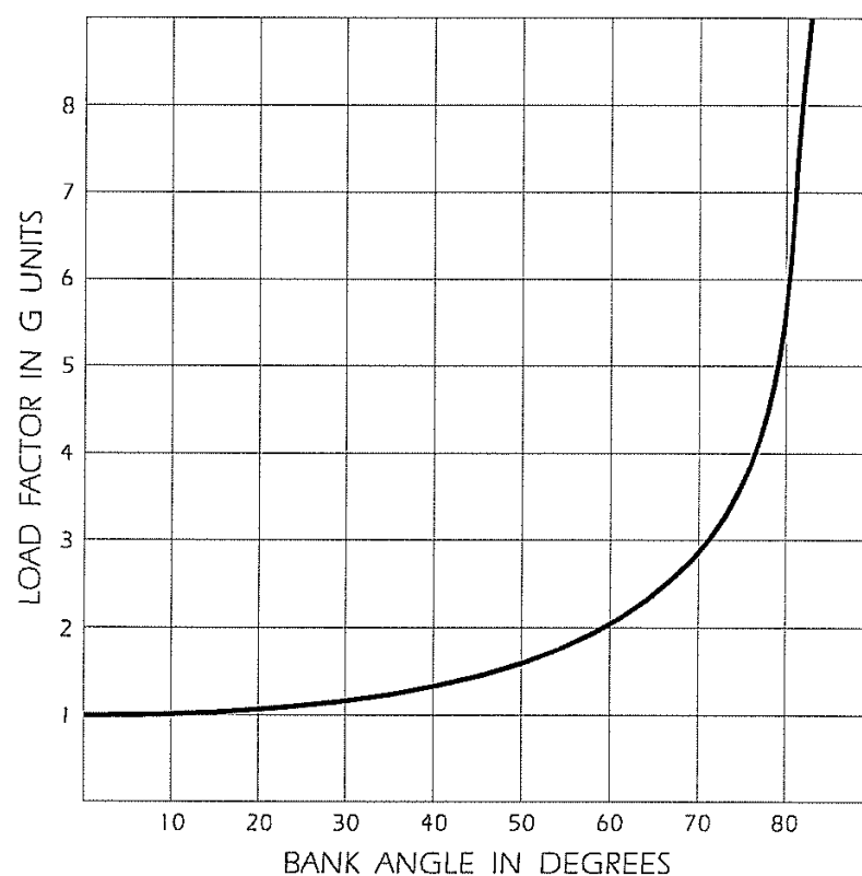
LOAD FACTOR CHART
